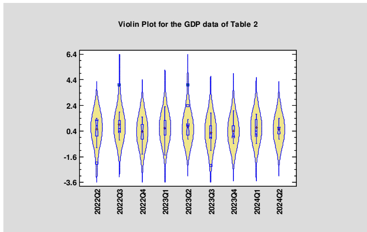
Fig. 1: Violin plots for the dataset of Table 2.
